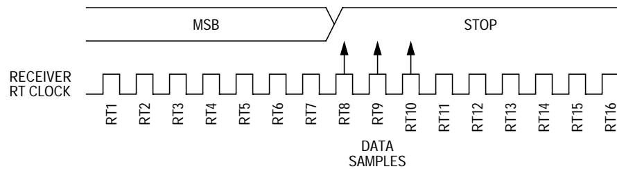
Figure 12-9. Slow Data
