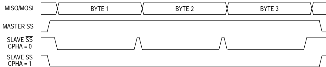
Figure 13-5. CPHA/SS Timing
